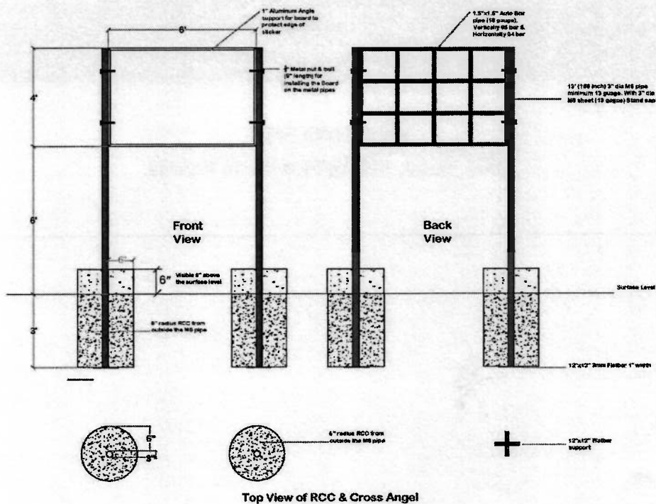
Detail diagram of AVCB Phase-III Signboard
