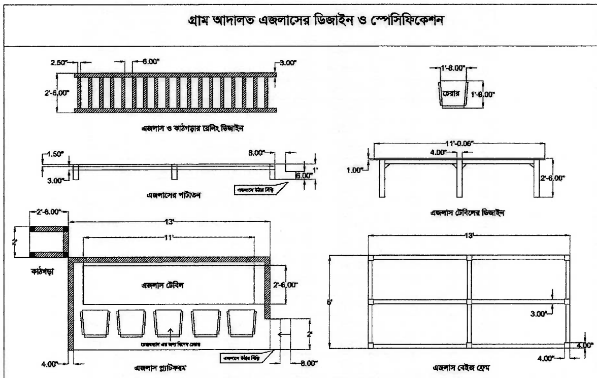
Detail diagram of AVCB Phase-III Ejlas
