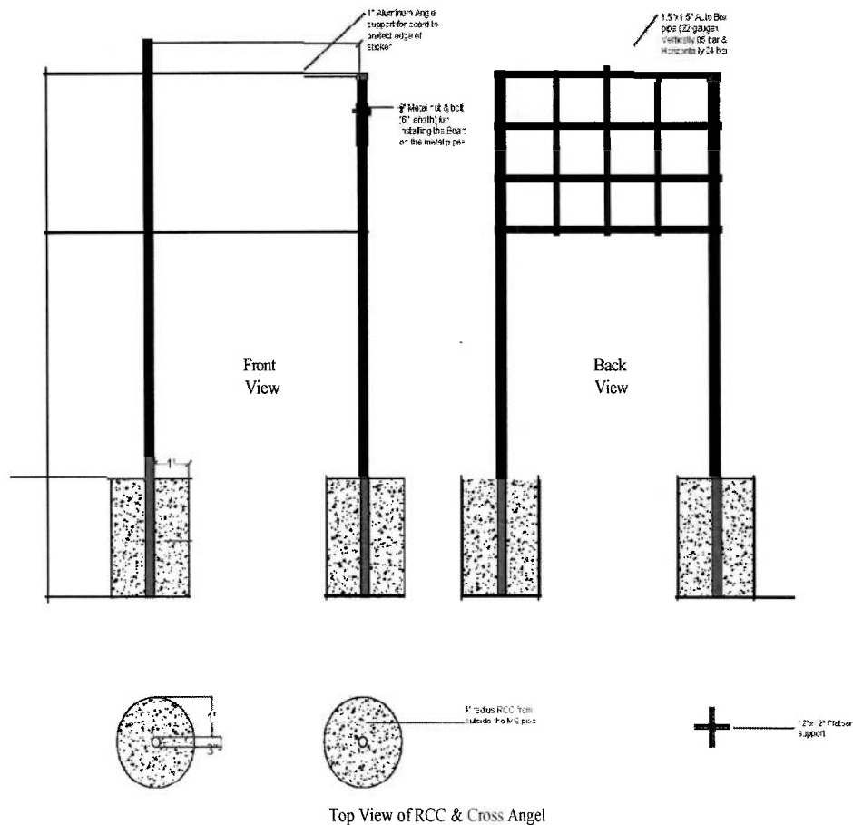
Detail diagram of AVCB Phase-III Signboard
